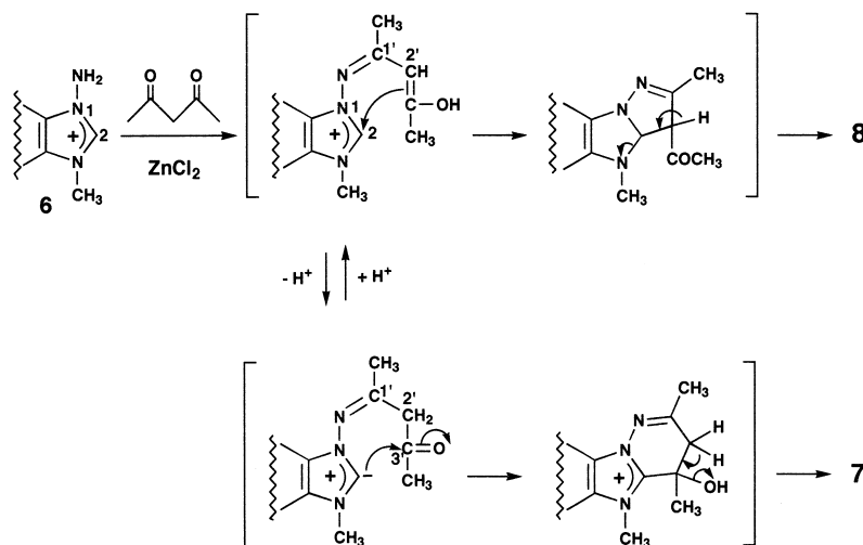
Scheme 4. Proposed reaction mechanisms.
