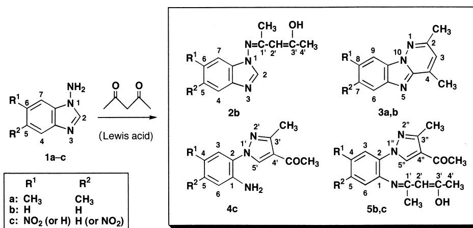
Scheme 2. Reactions of 1-aminobenzimidazole derivatives with 2,4-pentanedione.
