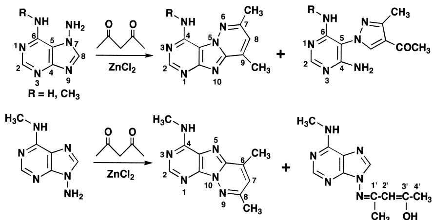
Scheme 1. Reactions of N -aminoadenines with 2,4-pentanedione.
