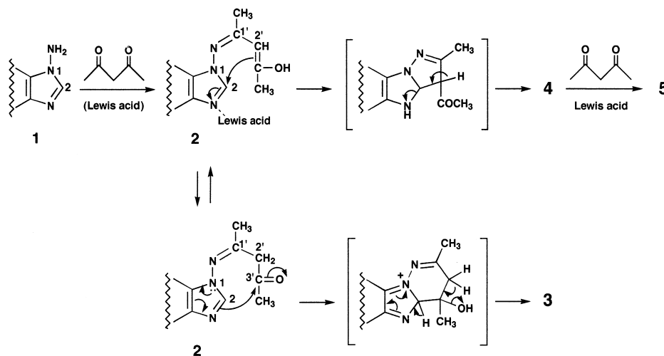
Scheme 3. Proposed reaction mechanisms.
